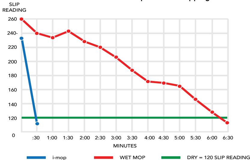
RELATIVE DRY TIMES: i-mop vs. Wet Mopping
